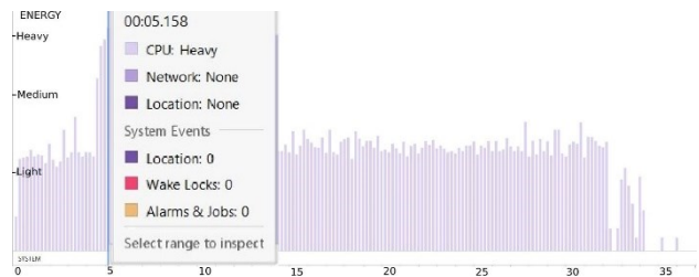
Figure 20. The amount of energy used by the application written with Xamarin
