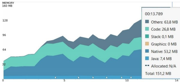
Figure 15. Memory rates used by the application written with Nativescript
